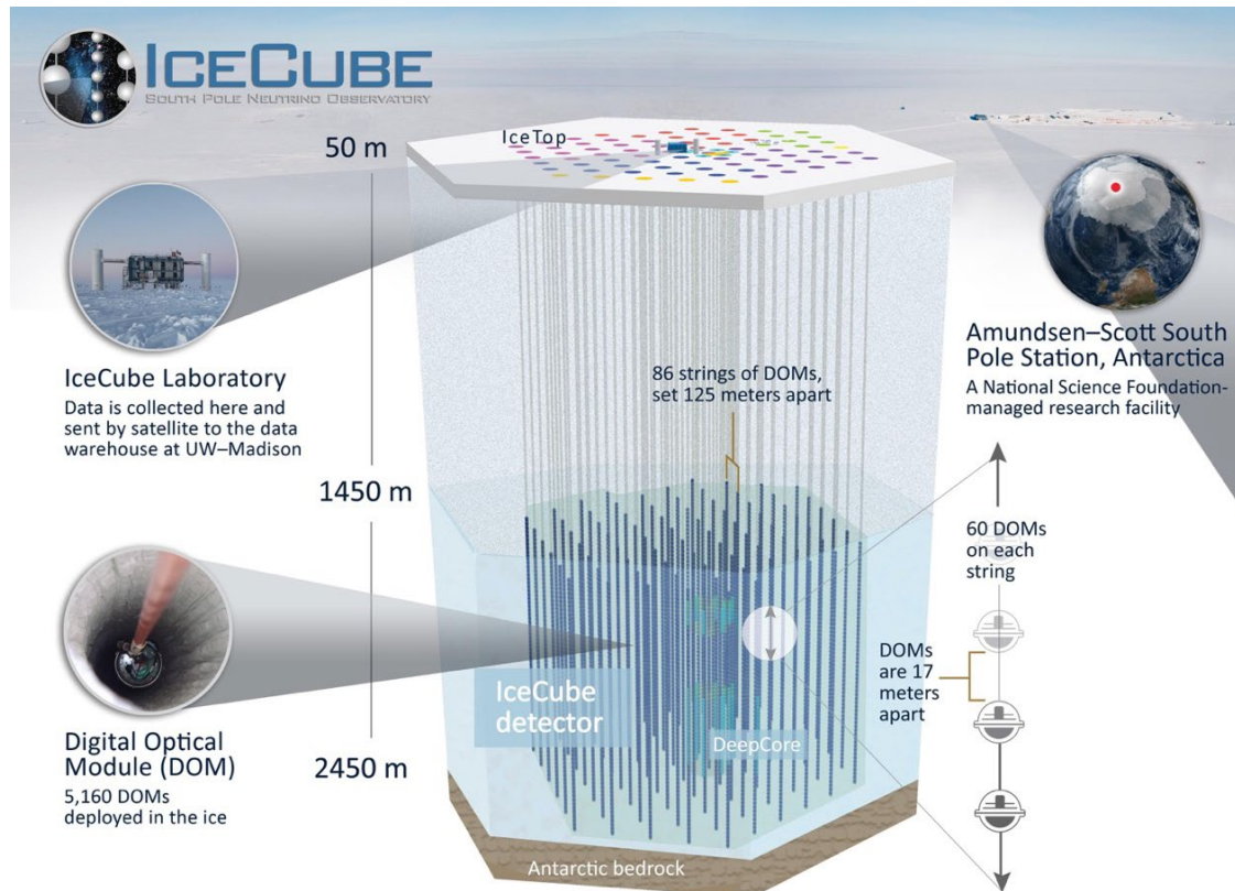
Figure 3. A schematic illustration of the IceCube Neutrino Observatory. Figure credit: IceCube Collaboration.
