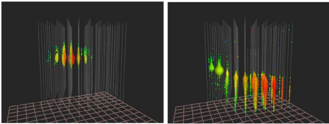
Figure 4: Left panel: The Cherenkov light signal produced by a cascade resulting from a neutral-current interaction of a neutrino of any flavour or a charged-current interaction of an electron or tau neutrino. The deposited energy is 1.14 PeV. Strings of optical sensors are marked as vertical lines of white dots. The colour codes the arrival time from red (early) through the rainbow to purple (late), while the size of the “blob” represents the number of Cherenkov photons detected. Right panel: a muon track that traverses IceCube from 11^\circ below the horizon. The deposited energy is 2.6 PeV. Figure credit: IceCube Collaboration.
