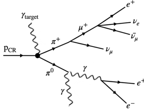
Figure 1. A schematic illustration of the production of charged ( \pi^+ ) and neutral pions ( \pi^0 ) in a p+\gamma interaction. The decay of charged pions yields neutrinos, whereas neutral pion decay yields gamma-rays.
