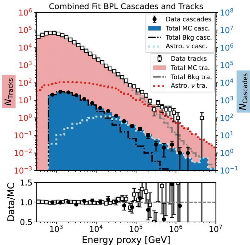
Figure 5. The energy distribution of cascade and track events, with contributions from astrophysical (Astro.) neutrinos [assuming the best-fit broken power-law (BPL) spectrum], total Monte Carlo (MC) background (Bkg) (atmospheric neutrinos and muons), and the total contribution from data. Note the different scales for tracks (left axis) and cascades (right axis). The energy proxy represents the energy reconstructed for the given event type. Figure credit: IceCube Collaboration, Physical Review Letters 136 (2026) 121002.
