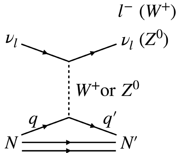
Figure 2. A neutrino of any flavour ( \nu ) interacts with a nucleon ( N ) in the detection medium (time flows from left to right). In such deep inelastic scattering events, the neutrino transfers momentum to the nucleon, causing it to dissociate ( N' ), yielding a hadronic cascade in the ice. The cascade particles give rise to Cherenkov light. In the case of a charged current interaction (mediated by a W^+ boson), the neutrino interaction yields a charged lepton ( l^- ) of the same flavour as the neutrino. This lepton also produces a Cherenkov light signal. If instead a neutral current interaction takes place (mediated by a Z^0 boson), there is no additional production of Cherenkov light, since the final-state neutrino is electrically neutral.
