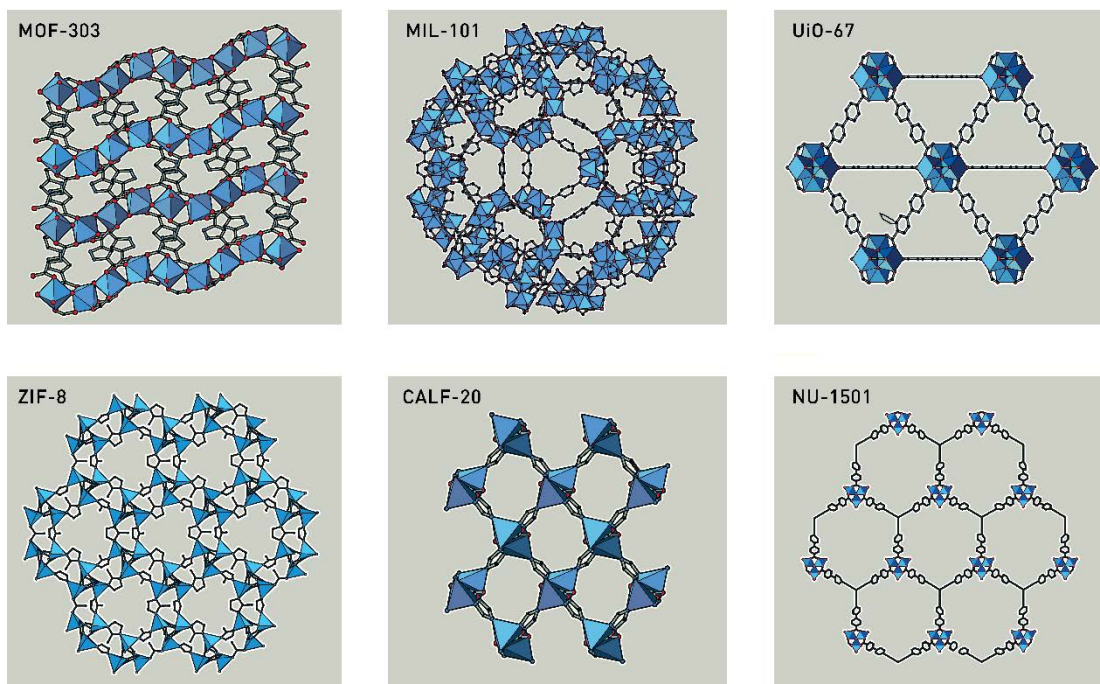
Figure 8: Examples of framework structures: MOF-303 has been applied in water adsorption from low-humidity air; 62 MIL-101 has large cavities and has been used in catalysis and in storage of H 2 and CO 2 ; 63–65 UiO-67 has been used to absorb PFAS from water; 66,67 ZIF-8 has been evaluated for mining rare-earth metals from wastewater; 68–70 CALF-20 can capture CO 2 ; 60 NU-1501 has been developed to store H 2 . 71
